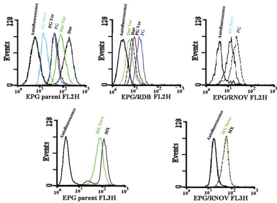
SUPPLEMENTARY FIG. S1. Accumulation analysis of daunorubicin, mitoxantrone, and prodigiosin in EPG85-257, EPG85-257RDB, and EPG85-257RNOV cells in the absence and presence of specific inhibitors. Dnr, daunorubicin; PG, prodigiosin, MX, mitoxantrone; Ver, verapamil; Novo, novobiocin.
