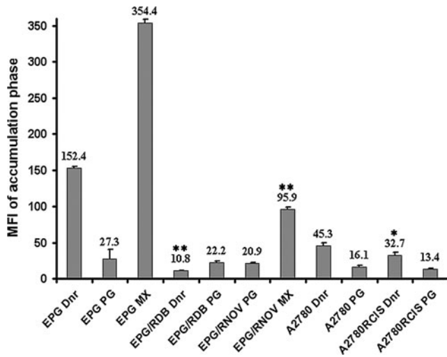
FIG. 4. FACS analysis of accumulation of daunorubicin, mitoxantrone, or prodigiosin in three individual experiments in a panel of parental and their resistant cell lines. Values are presented as the mean ± SE. The symbols (** and *) represent the mean fluorescence difference between parental and resistant cells with p < 0.001 and p < 0.05 , respectively. Dnr, daunorubicin; PG, prodigiosin; MX, mitoxantrone.
